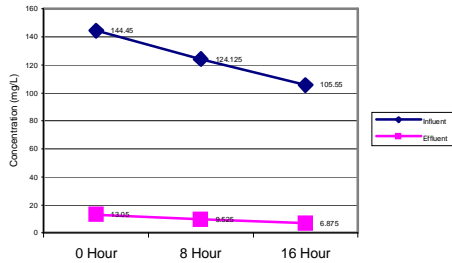
Average BOD 5 Characteristics during Dynamic Operation
